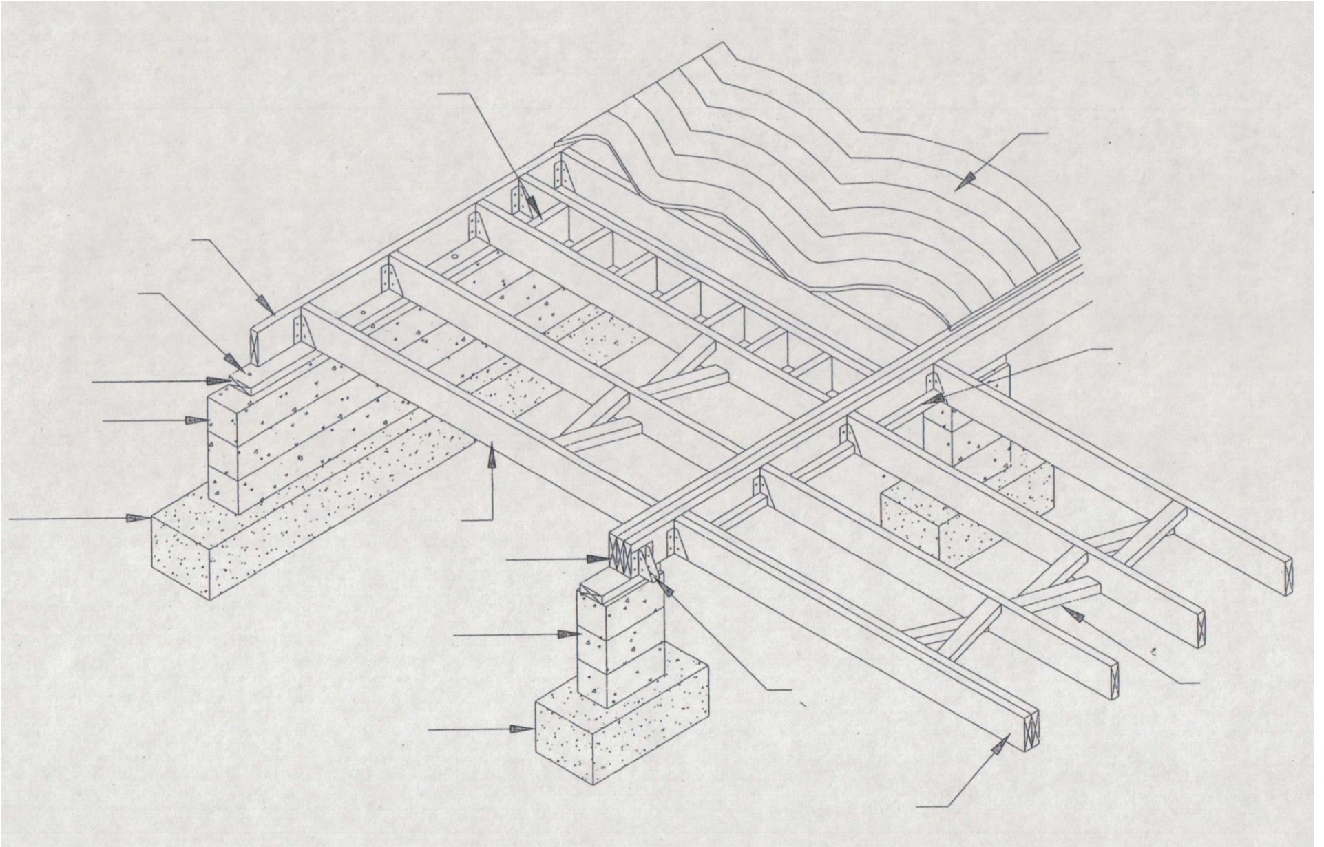
FLOOR FRAMING DETAIL
