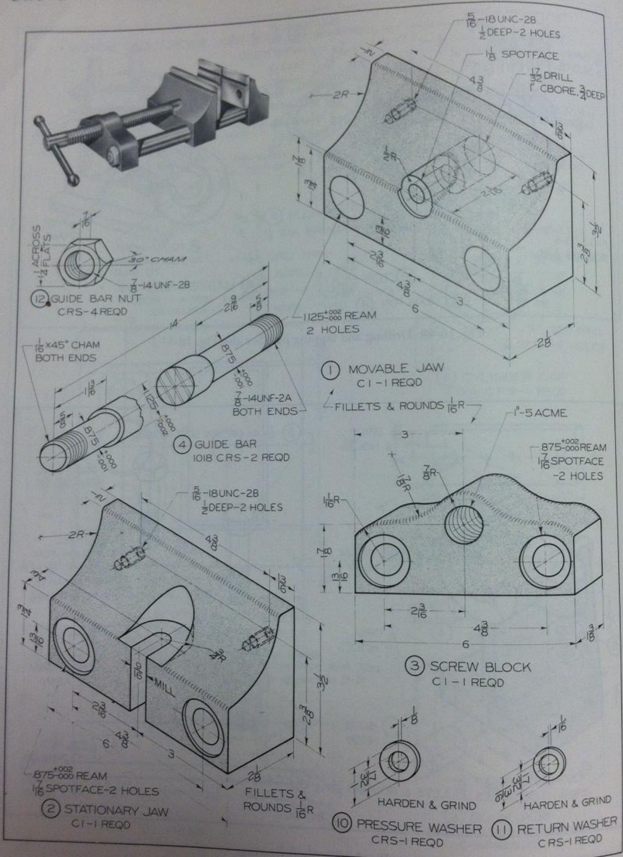
Fig. 16-50. Drill press vise. (See also Fig. 16-51.)
